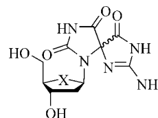
Figure 1. 2'-Deoxyspiroiminodihydantoin (X = O; dSp) and its carbocyclic analog (X = CH 2 ; cdSp).
