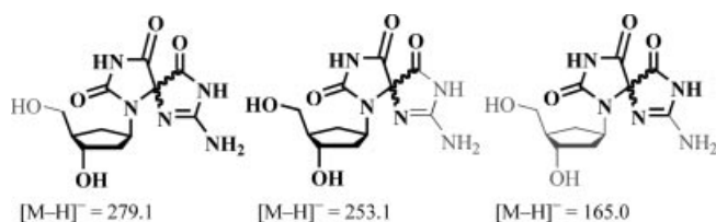
Figure 3. Negative-mode ESI-MS/MS of 7 at 35 eV. Structural assignments of the fragmentations are suggested as indicated in bold.
