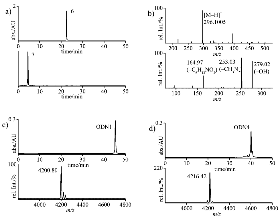
Figure 2. a) HPLC of 6 and 7 using a gradient of 0–25% buffer B in 45 min; buffer A: 2 mM TEAA in water; buffer B: 2 mM TEAA in 80% acetonitrile. b) Negative ESI-MS (top) and MS/MS (bottom); parent ion of 7 [M-H]^- : m/z = 296.1005. c) HPLC and MALDI-TOF of ODN1. d) HPLC and MALDI-TOF of ODN4; buffer A: 0.1 M TEAA in water; buffer B: 0.1 M TEAA in 80% acetonitrile (c and d).
