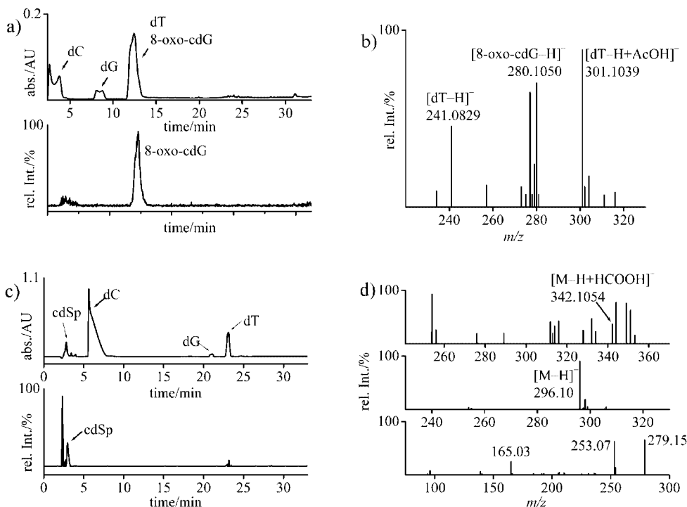
Figure 4. LC-MS and LC-MS/MS of enzymatic digest of: a) ODN1 , HPLC on Macherey–Nagel Nucleodur 125-2 3 \mu C18 pyramid, 2 mM TEAA, pH = 7.0, in water (A) and 80% acetonitrile (B), 100% A 10 min, 0–10% B 18 min, UV trace (top) and ion count at m/z = 295.5–296.5 (bottom); b) ESI-MS of peak eluting at 12 min; c) ODN4 , HPLC on Uptisphere Interchrom, 2 mm ammonium formate, pH = 5.5, in water (A) and 80% acetonitrile (B), gradient equal to a), UV trace (top), ion count at m/z = 341.5–342.5 (bottom); d) ESI-MS (top), -MS/MS (centre) and -MS/MS/MS (bottom) of peak eluting at 3 min, parent ions are [M - H + HCOOH]^- : m/z = 342.1054 for MS/MS and [M - H]^- : m/z = 296.10 for MS/MS/MS; M = cdSp.
