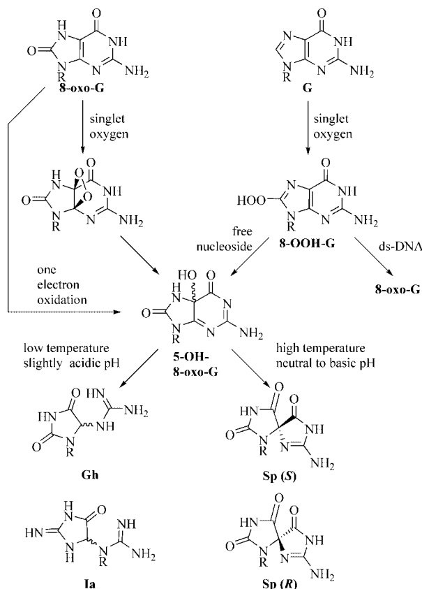
Scheme 1. Short overview of the oxidation of G and 8-oxo-G to guanidinohydantoin Gh and spiroiminodihydantoin Sp. Iminoallantoin (Ia) has not yet been identified as 1 O 2 oxidation product of 8-oxo-G. R = β-D-ribofuranosyl, 5-OH-8-oxo-G = 5-hydroxy-8-oxo-7,8-dihydroguanosine, 8-OOH-G = 8-hydroperoxyguanosine.
